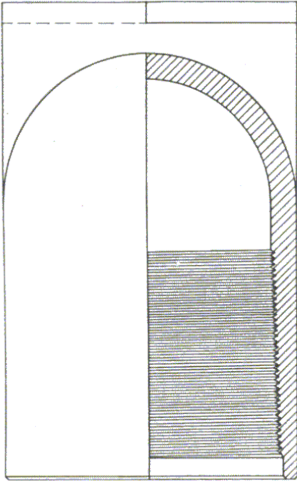
Fig.15 : Coupling/Centralizer Fin
