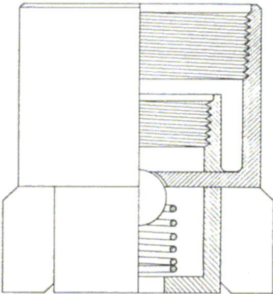
Fig.16 : Wash Down Shoe
