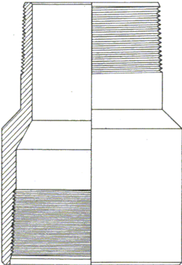
Fig.14 : Bull Plug
